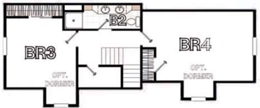
SUGGESTED SECOND FLOOR LAYOUT (SITE CONSTRUCTED)
